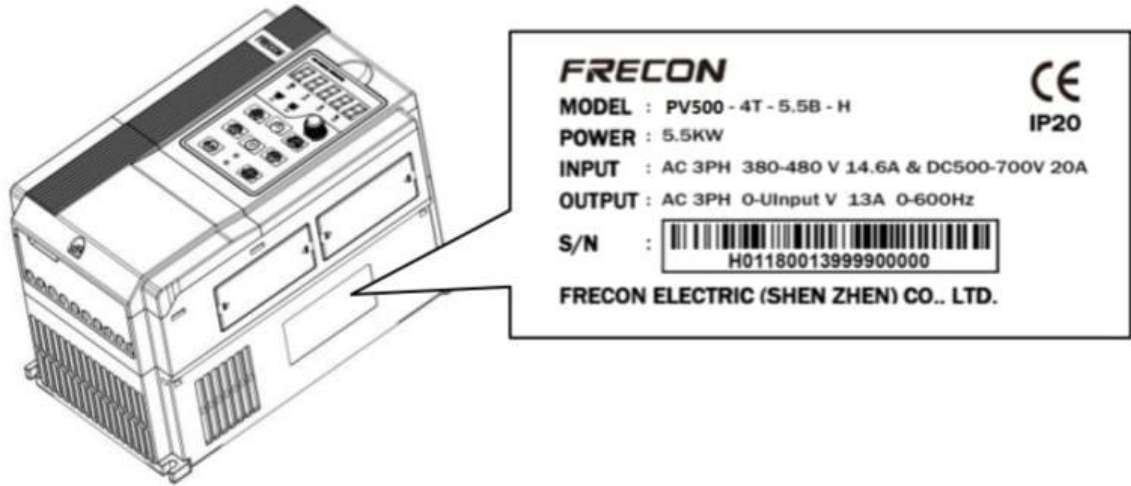
Figure 1-1 Name Plate
